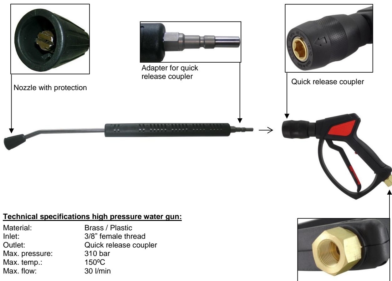
3/8" female thread
